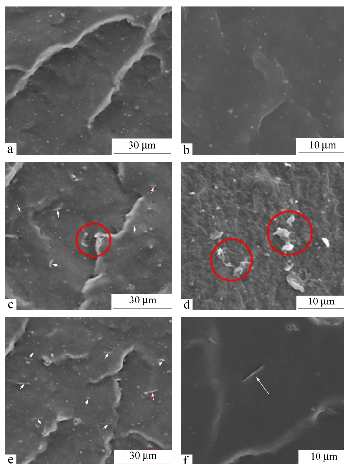
Fig. 5 FESEM images of neat NR (a, b), NR/GO-2.12 (c, d) and NR/MLPB-GO-2.12 composite (e, f). White arrows indicate the GO sheets embedded in the matrix and circles present the aggregates of GO sheets.
