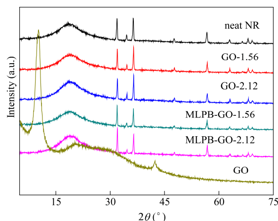
Fig. 7 XRD patterns of GO, neat NR, NR/GO and NR/MLPB-GO composites
